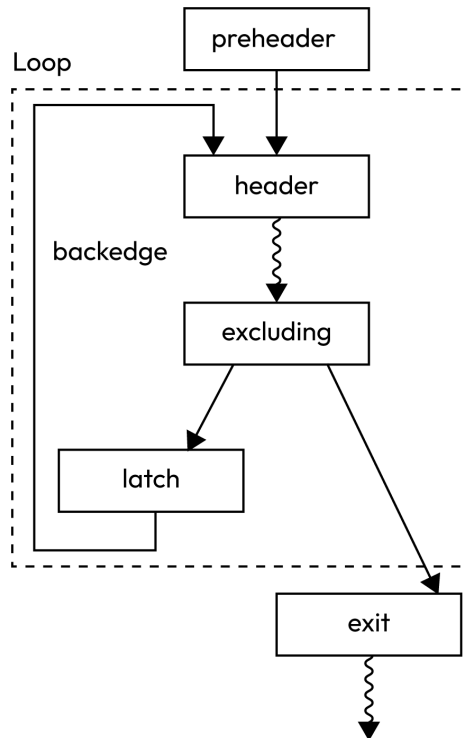
Figure 4.6: A canonical loop in LLVM
